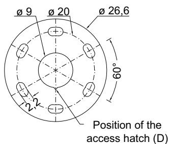
Flange plan Scale 1:10
